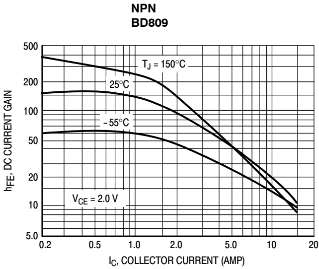
Figure 3. DC Current Gain
