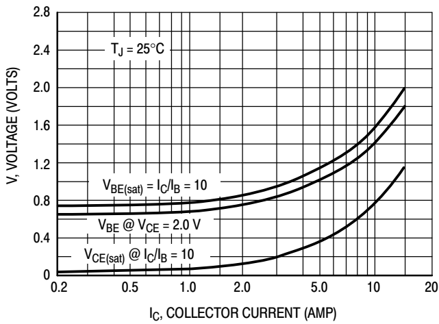
Figure 5. "On" Voltages
